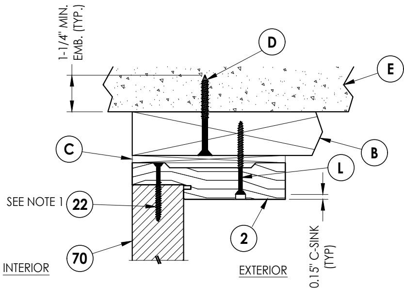
1 5 VERTICAL CROSS SECTION Shown w/ 2X Buck Inswing shown (Outswing similar)
