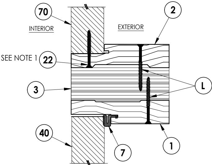
3 5 VERTICAL CROSS SECTION Shown w/ 2X Buck Inswing shown (Outswing similar)
