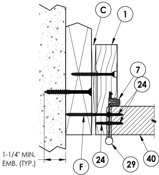
2 5 HORIZONTAL CROSS SECTION Shown w/ 2X Buck Inswing shown (Outswing similar)
