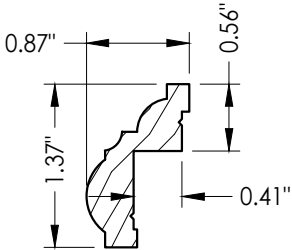
GLAZING BEAD
